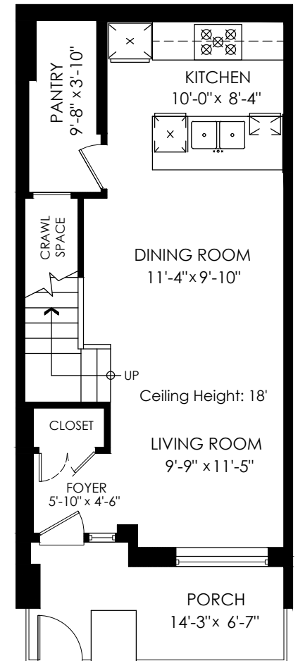
Main Floor Plan Floor Area: 463 sq.ft. Ceiling Height: 7'-6" Crawl Space: 22 sq.ft.
