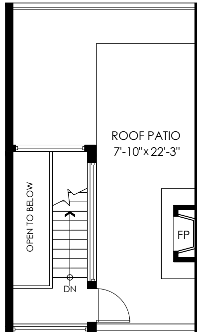
Rooftop Floor Plan Stair Area: 69 sq.ft. Rooftop Patio: 175 sq.ft.
