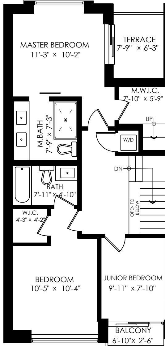
Upper Floor: 768 Sq.Ft. Ceiling Height: 8'-5"
